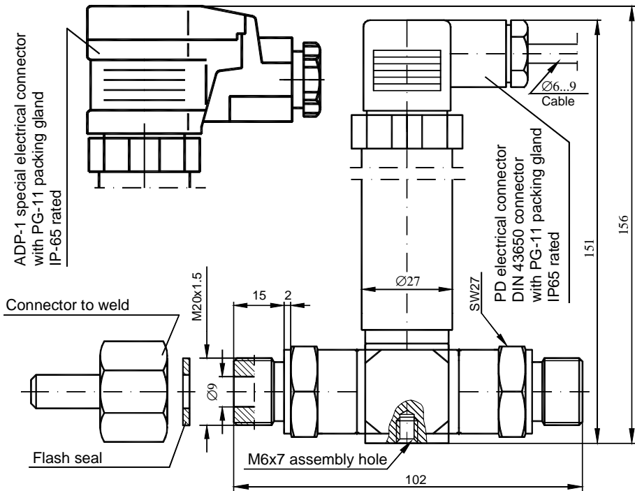
Fig.1. AS-dP series differential pressure transmitter.
