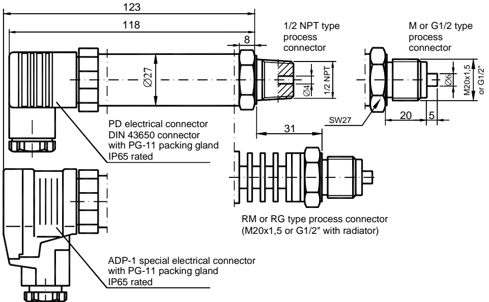
Fig.1. AS series pressure transmitter.
