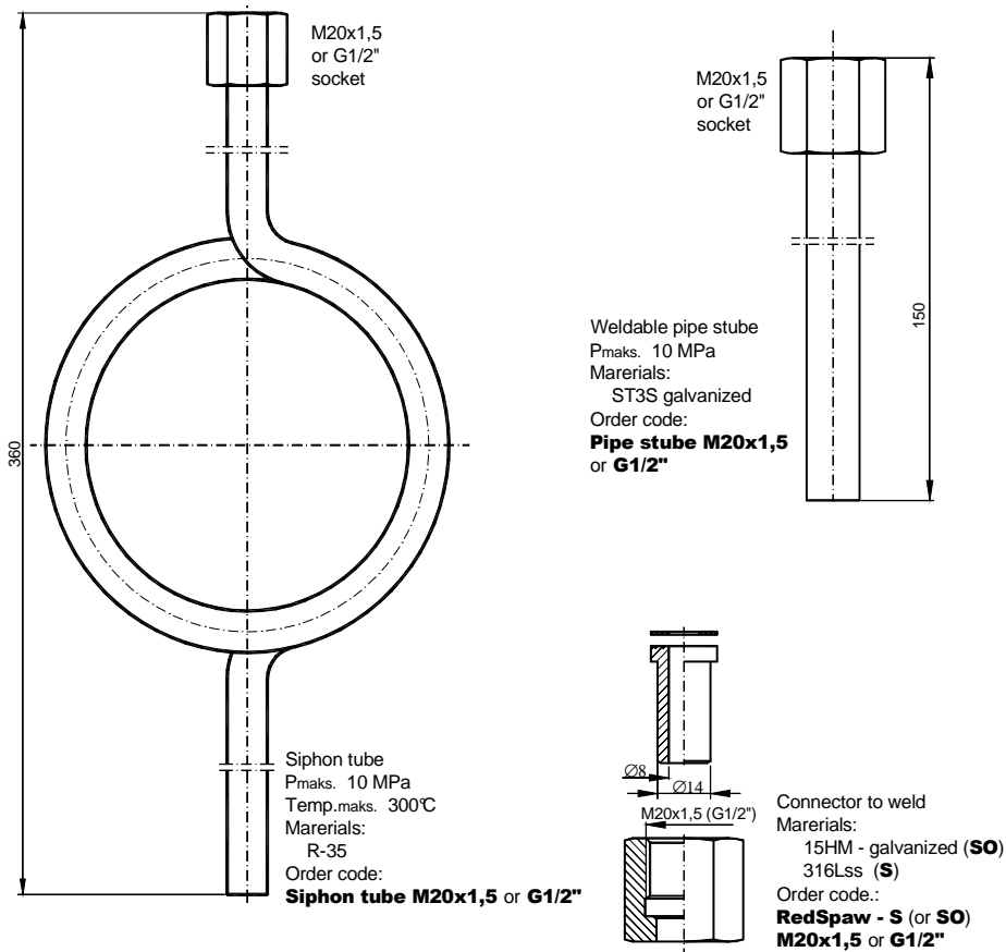
Figure 15. Additional equipment for fitting of pressure transmitters.
