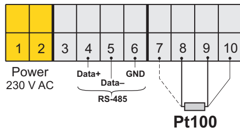
Electrical connection diagram
